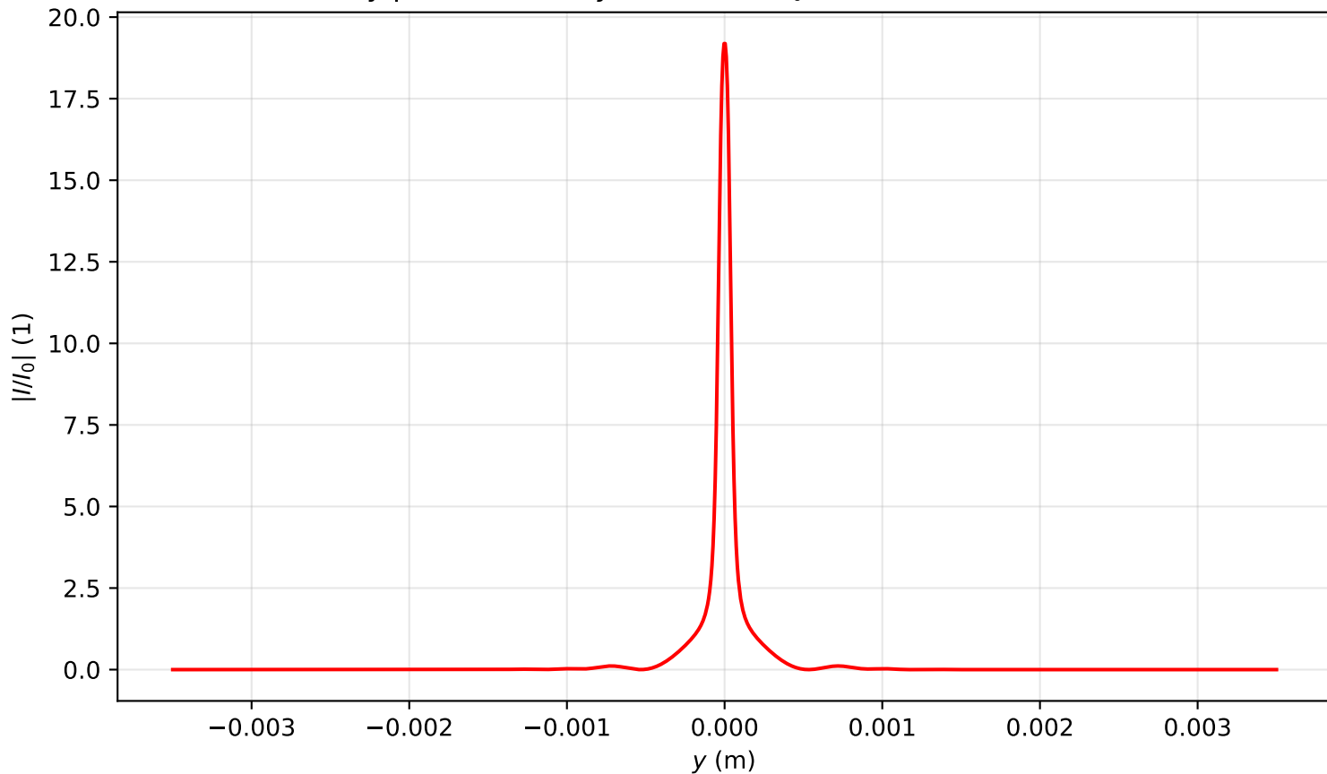
Intensity profile I(x=0, y, z=0.955)/I_0 , P_{in}=5.5P_{cr} , artificial time
